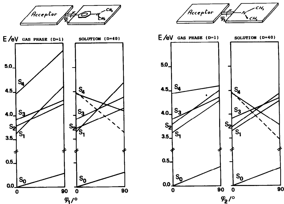
Figure 7. Effect of the solvent polarity on the energy correlation diagrams for the lowest-lying singlet states of DCS in the planar and 90° twisted conformations of the dimethylanilino ( \phi_1=90^\circ ) and dimethylamino ( \phi_2=90^\circ ) groups. Dotted lines show the effect of using R^{eff} = 3 a.u. instead of 4 a.u. in eq. (1).
