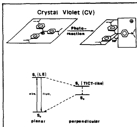
Figure 3. Model of the excited - state relaxation of Crystal Violet [7] involving a low-lying non-fluorescent TICT-like state.
