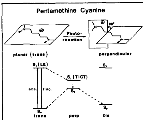
Figure 4. Model of the excited-state relaxation of a polymethine cyanine [9] involving trans \rightarrow cis isomerization via a low-lying TICT-like state.
