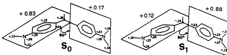
Figure 12. Charge distributions in the S_0 and S_1 states of twisted ( \phi=90^\circ ) MHB.
